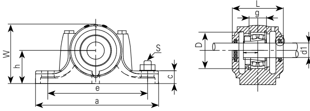
DATA TABLE - S(S)N3000 / S(S)N3100 PLUMMER BLOCK
